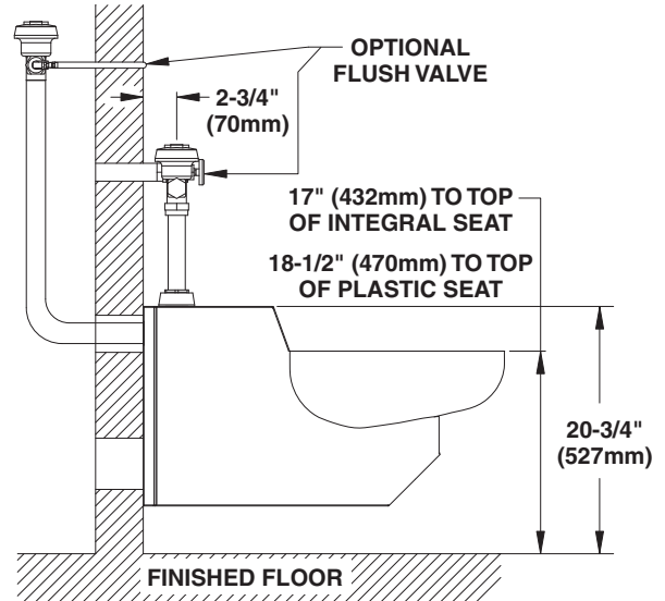
Dimensions - Side View
