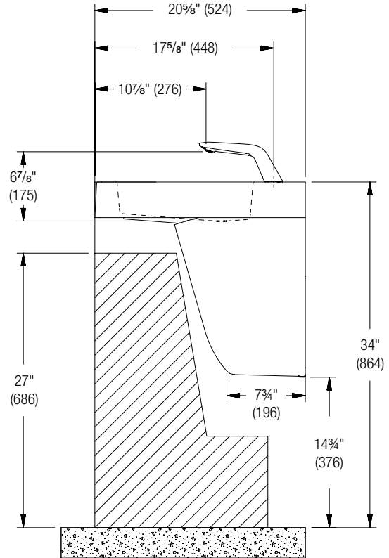
Standard Height (ADA) – WBD1
