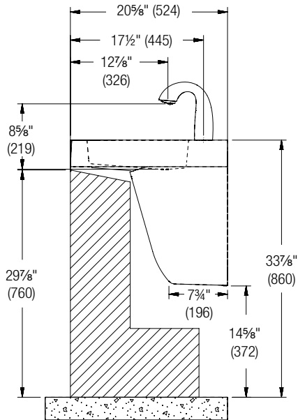
OBC Height – Verge Faucet
