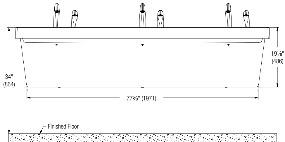
Front View (shown with Verge Soap & Faucet)
